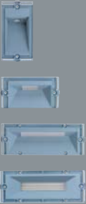
Quantum masks
